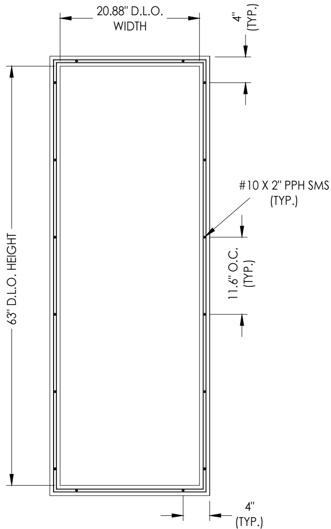
4A ALUMINUM LITE FRAME** (w/ 1-1/4" Glazing)
